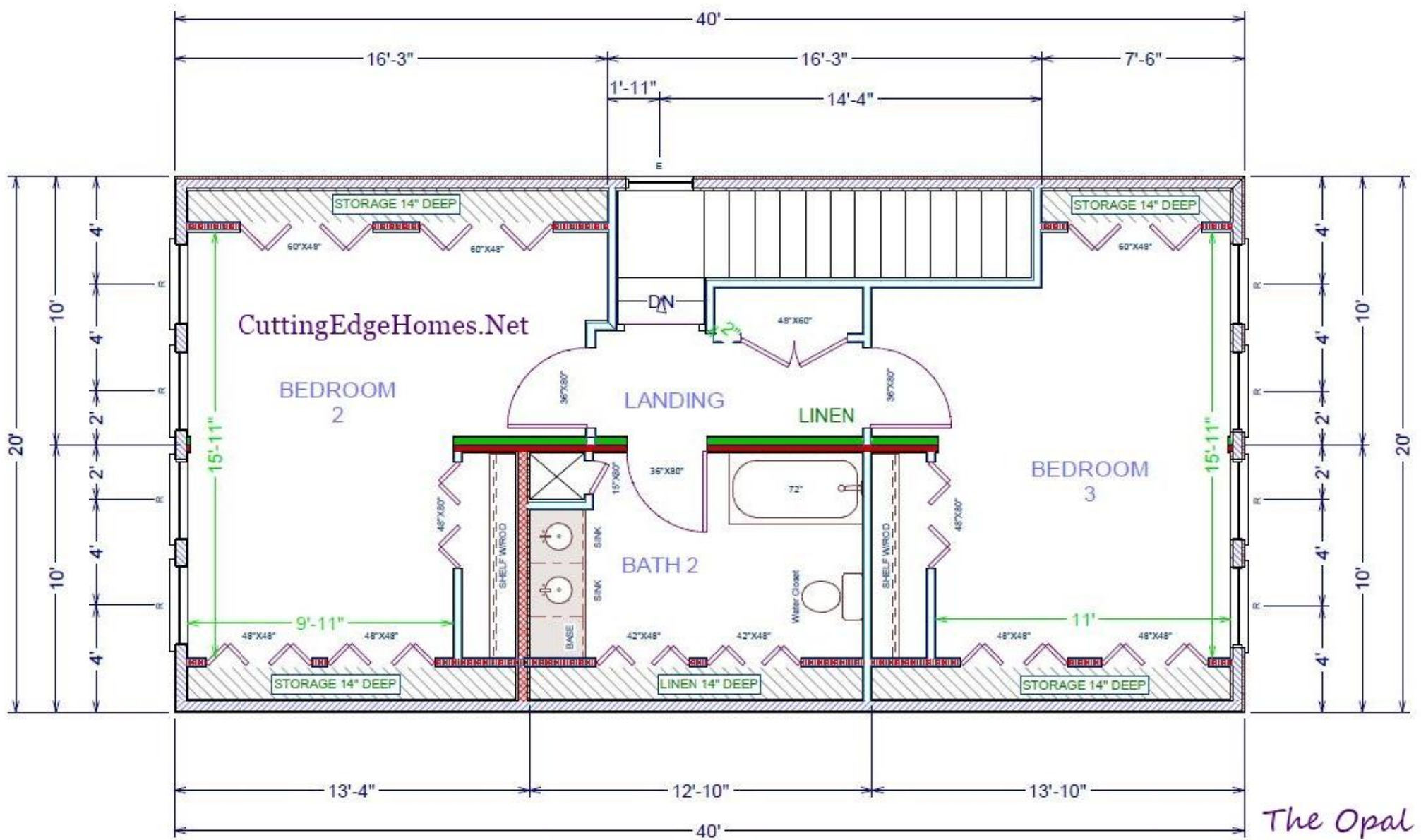
Plan as drawn has 4' sidewalls on the second floor, not a standard specification.
